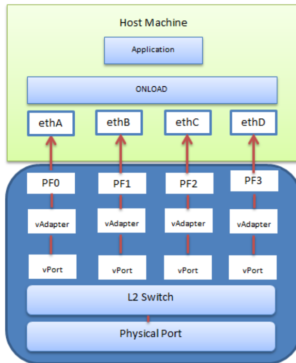
Figure 18: Onload and NIC Partitioning
