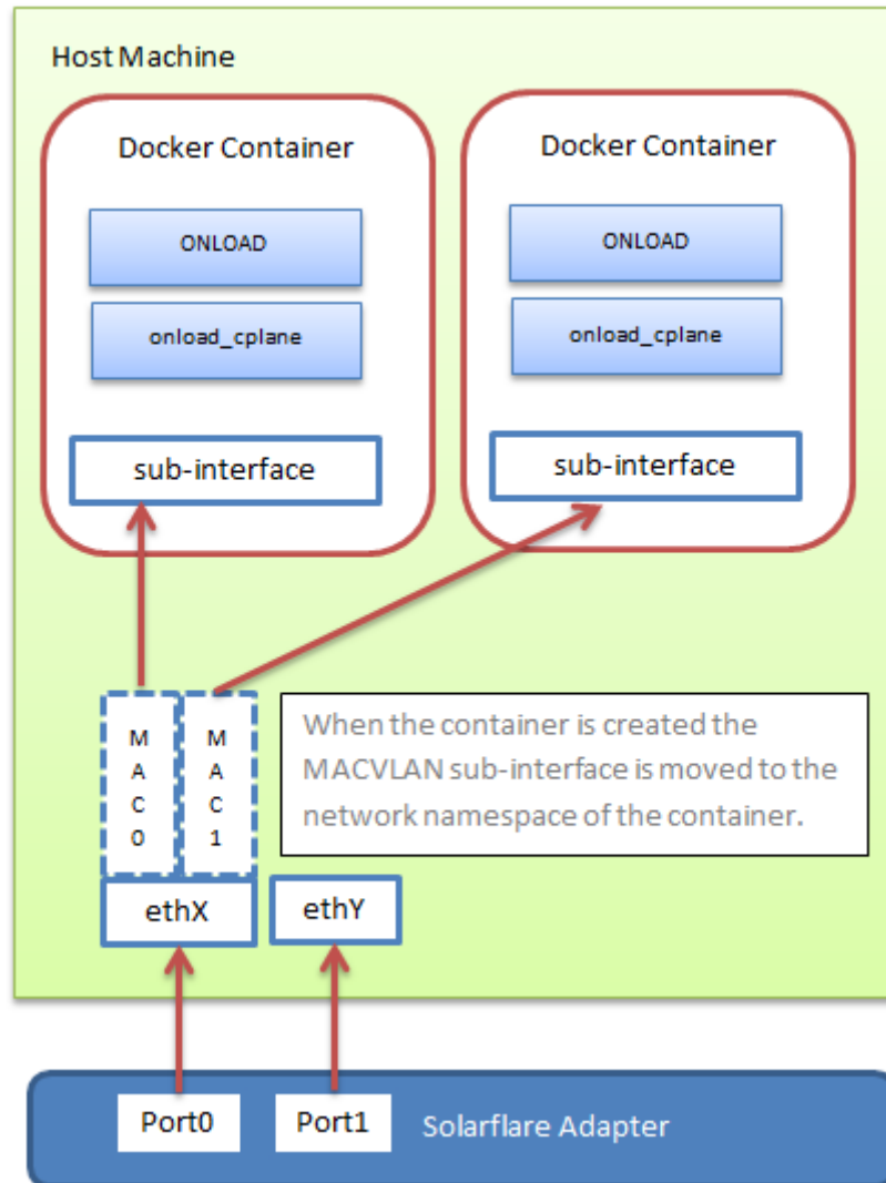
Figure 20: Onload using MACVLAN sub-interfaces
