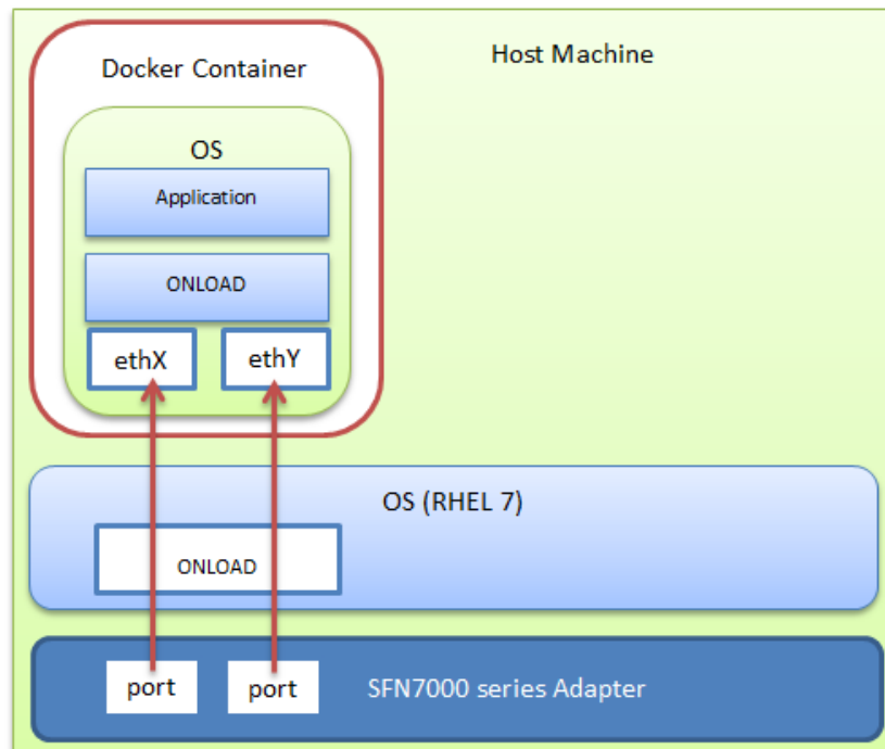
Figure 19: Onload in a Docker Container
