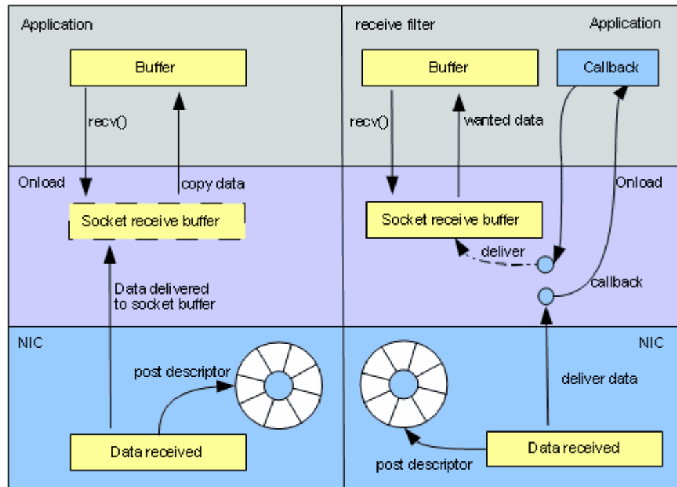
Figure 32: UDP Receive Filtering
