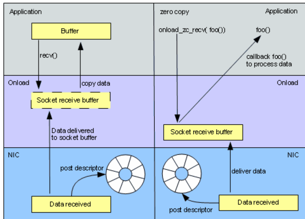
Figure 22: Traditional vs. Zero-Copy UDP Receive
