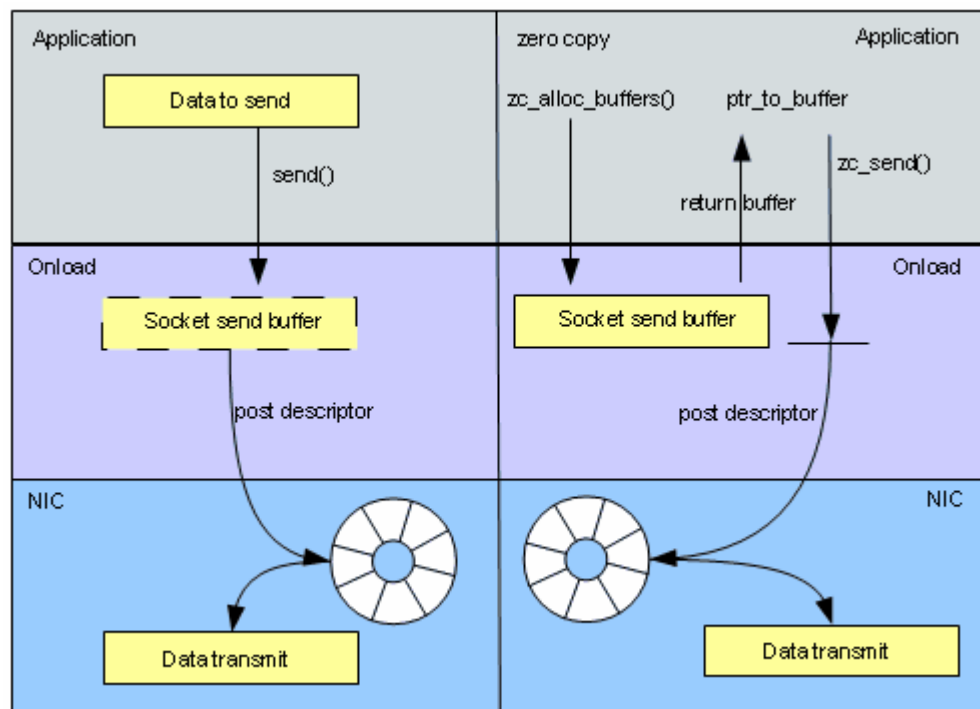
Figure 26: Traditional vs. Zero-Copy TCP Transmit
